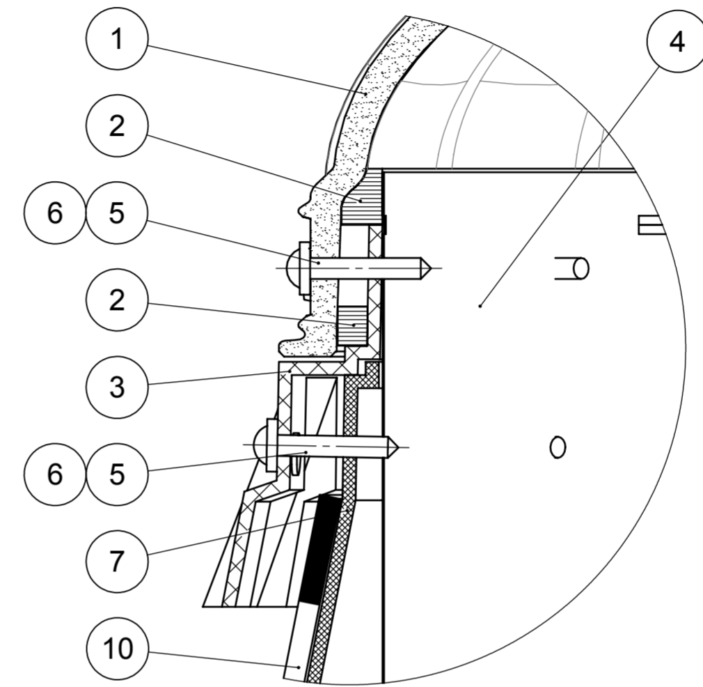
DETAIL A DOME FIXATION
