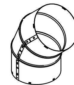
ADJUSTABLE ELBOW 45°
